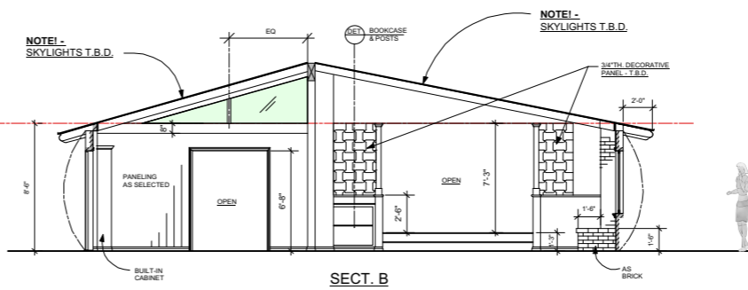
SECT. B
