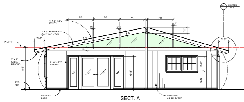
SECT. A
