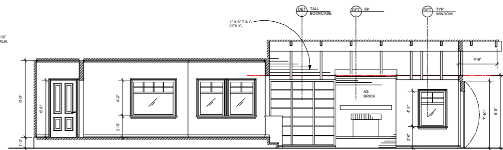
SECT. D
