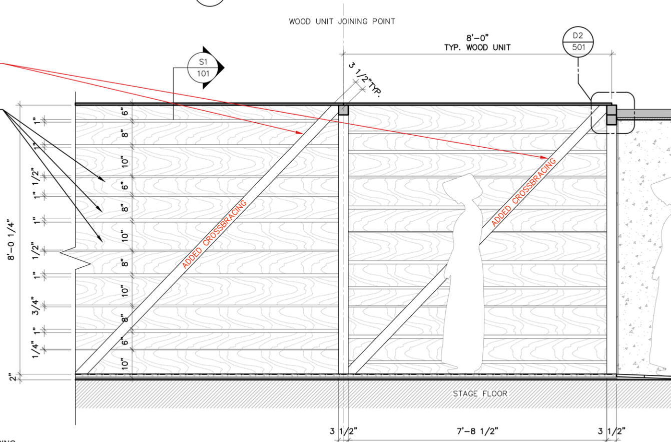
V1 VIEW - CROSS BRACING RUNNING IN SAME DIRECTION FOR EVERY UNIT SCALE: NTS
