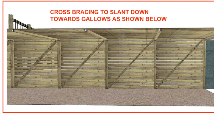
V2 VIEW - SECTION SHOWING CROSS BRACING SCALE: NTS
