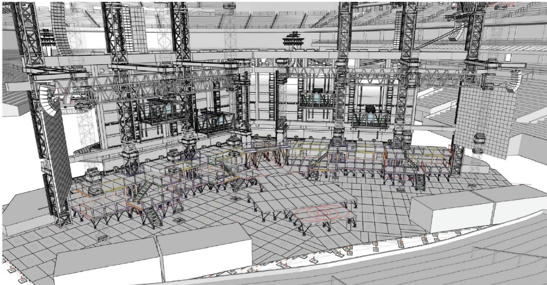
PROJECT XX - 2018 - REAR PERSPECTIVE ISO - ROOF SKIN REMOVED
