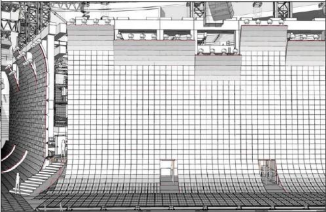
VIEW SL FRONT ELEVATION
