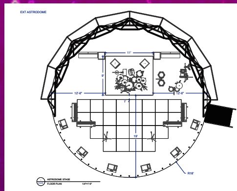
- ASTRODOME STAGE 214-00 FLOOR PLAN 1/4"=1'-0"
