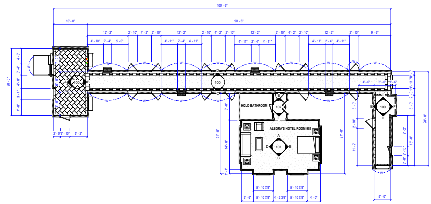
① 9th Floor Hallway Floor Plan 1/8" = 1'-0"
