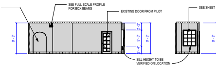
Ⓕ Hallway Elevation F 1/8" = 1'-0"
