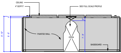
A Room 981 Elevation A 1/4" = 1'-0"
