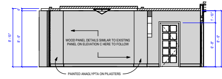
D Room 981 Elevation D 1/4" = 1'-0"
