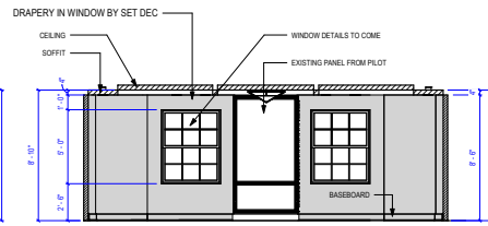
C Room 981 Elevation C 1/4" = 1'-0"
