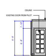
E Room 981 Elevation E 1/4" = 1'-0"
