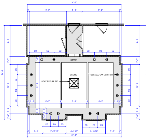
2 Room 981 Reflected Ceiling Plan 1/4" = 1'-0"
