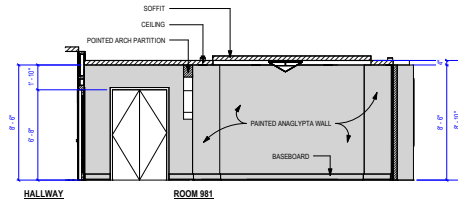
B Room 981 Elevation B 1/4" = 1'-0"
