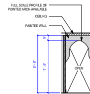
F Room 981 Elevation F 1/4" = 1'-0"
