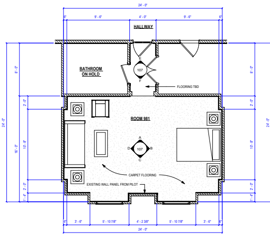
1 Room 981 Floor Plan 1/4" = 1'-0"
