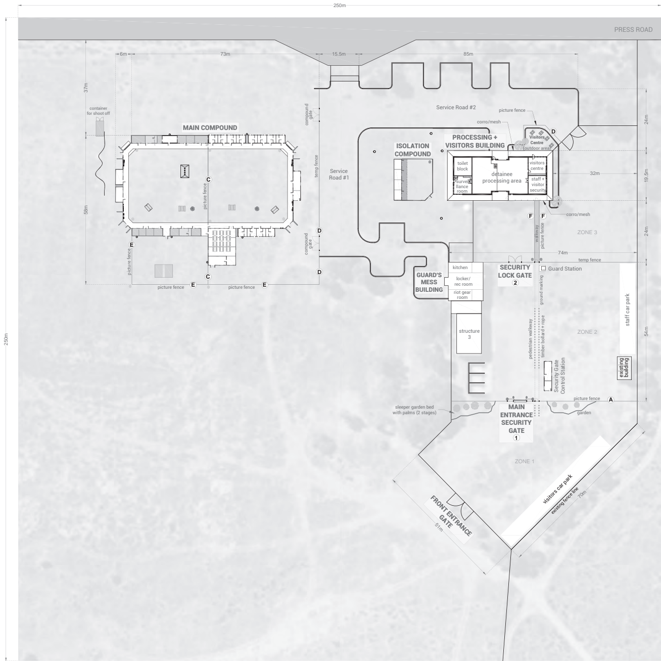
SITE PLAN Plan View Scale 1:500
