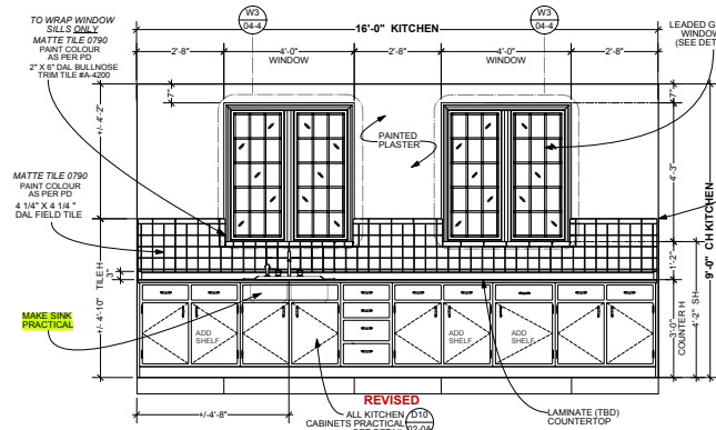
EK1 ELEVATION - INT. SCHLAFLY HOUSE - KITCHEN WALL 1 02-0 SCALE: 1/2" = 1'-0"
