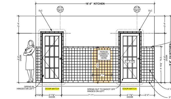
EK3 ELEVATION - INT. SCHLAFLY HOUSE - KITCHEN WALL 3 02-0 SCALE: 1/2" = 1'-0"
