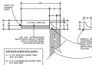
D-C DETAIL - KITCHEN DOOR CASING 02-0 SCALE: 1'-0" = 1'-0"
