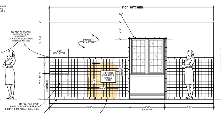
EK2 ELEVATION - INT. SCHLAFLY HOUSE - KITCHEN WALL 2 02-0 SCALE: 1/2" = 1'-0"
