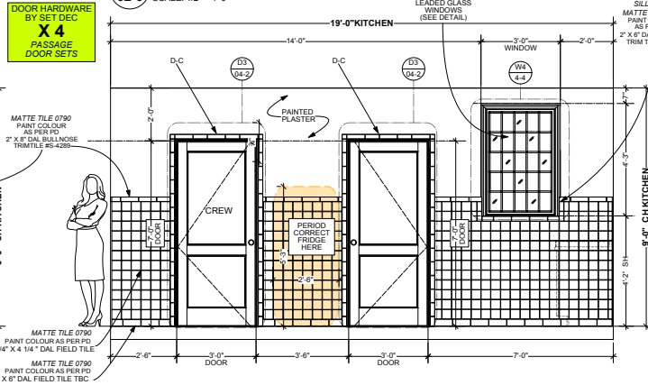
EK4 ELEVATION - INT. SCHLAFLY HOUSE - KITCHEN WALL 4 02-0 SCALE: 1/2" = 1'-0"
