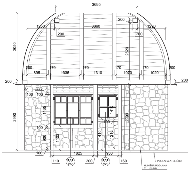
POHLED A_1:50 ELEVATION A_1:50
