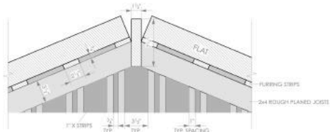
SECTION OF RIDGE BEAM SCALE 2" = 1'-0"
