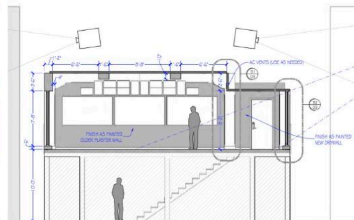
TACTICAL AUDITORIUM: SECTION "B" SCALE: 1/8" = 1'-0"
