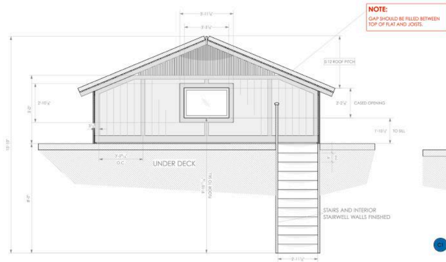
ELEVATED SECTION - BEDROOM SCALE 1/2" = 1'-0"
