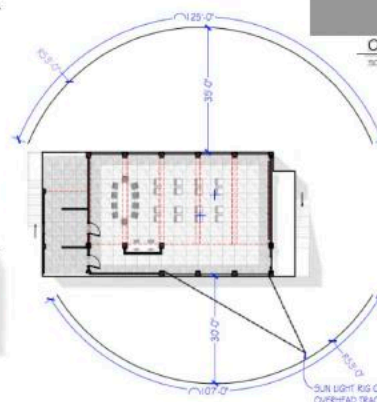
KEY PLAN: TACTICAL AUD. SCALE: 1/8" = 1'-0"
