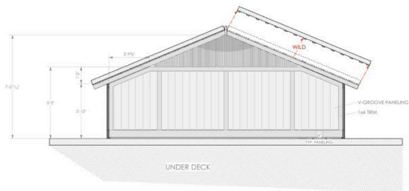
ELEVATED SECTION - BED ROOM SCALE 1/2" = 1'-0"
