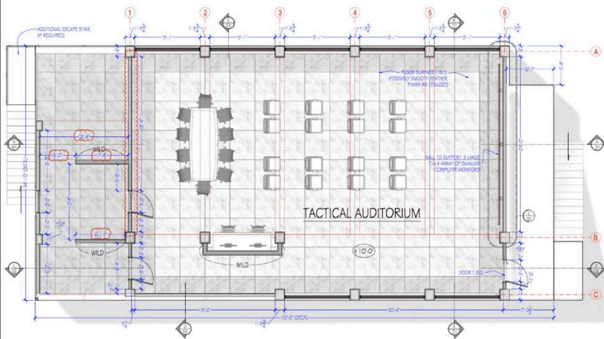
TACTICAL AUDITORIUM: PLAN SCALE: 1/8" = 1'-0"
