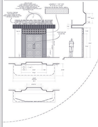
F5 PLAN OF OVERHANG COVER
