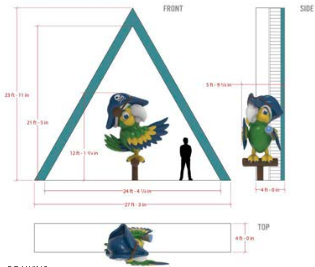
DRAWING
