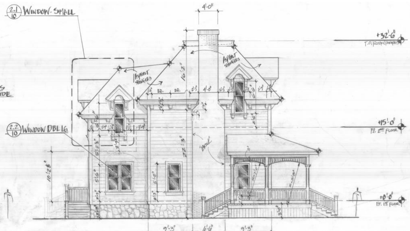
D LEFT VIEW Scale: 1/4" = 1'-0"
