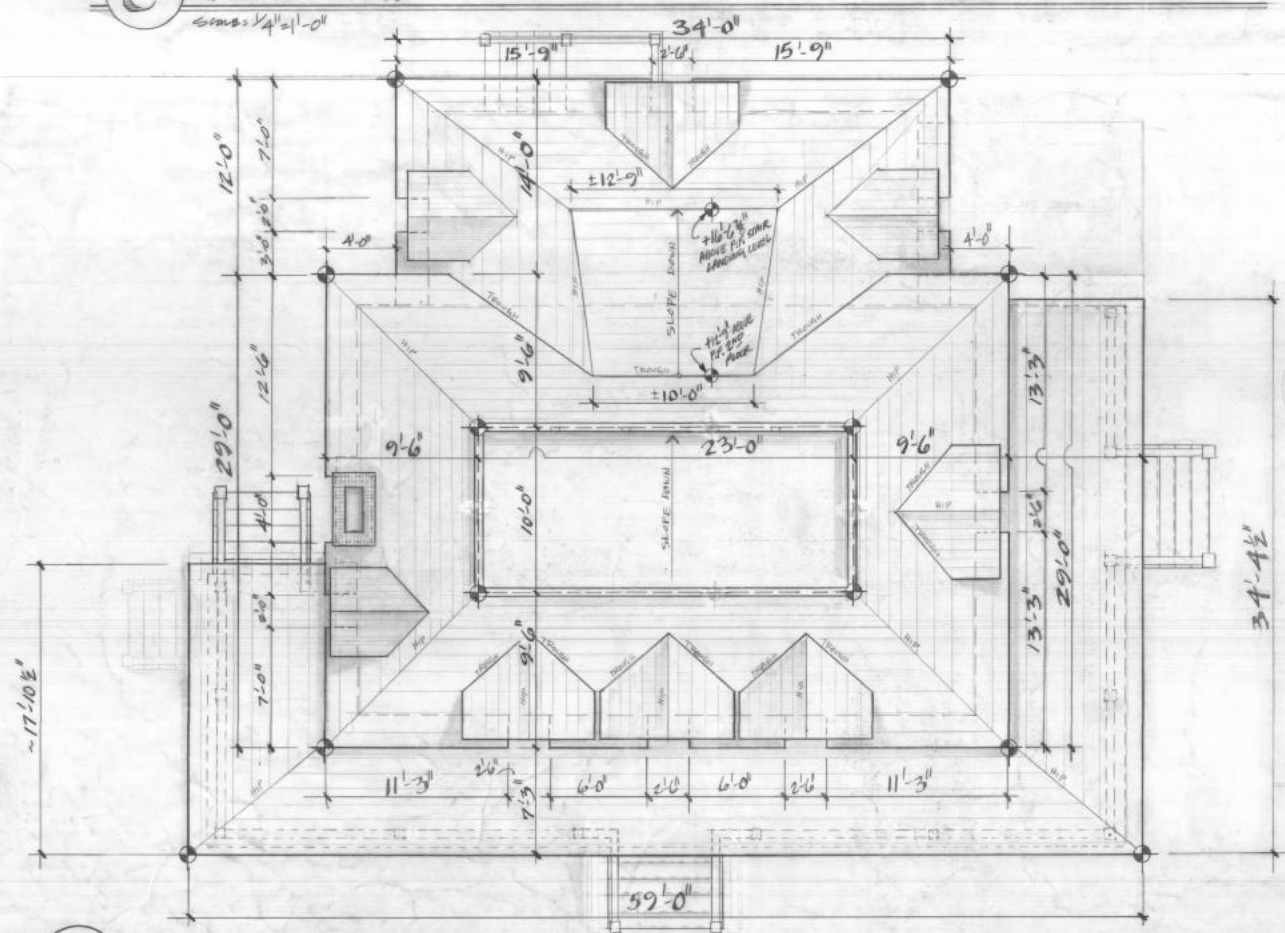
-4 ROOF PLAN Scale: 1/4" = 1'-0"
