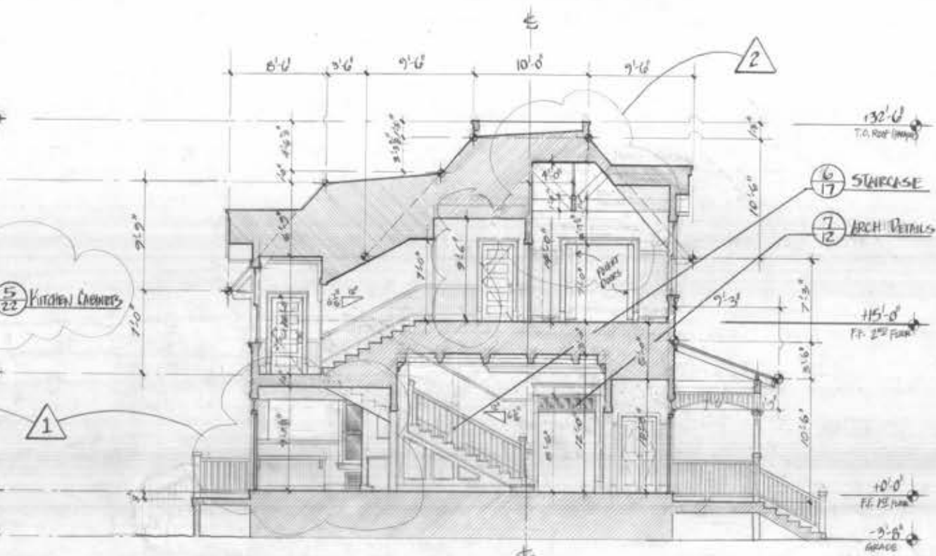
SECTION
