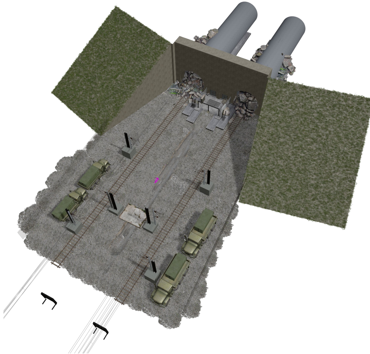
3D MODEL RENDER SHOWING TUNNEL EXIT OVERVIEW AND LAYOUT OF FINAL DESIGN
