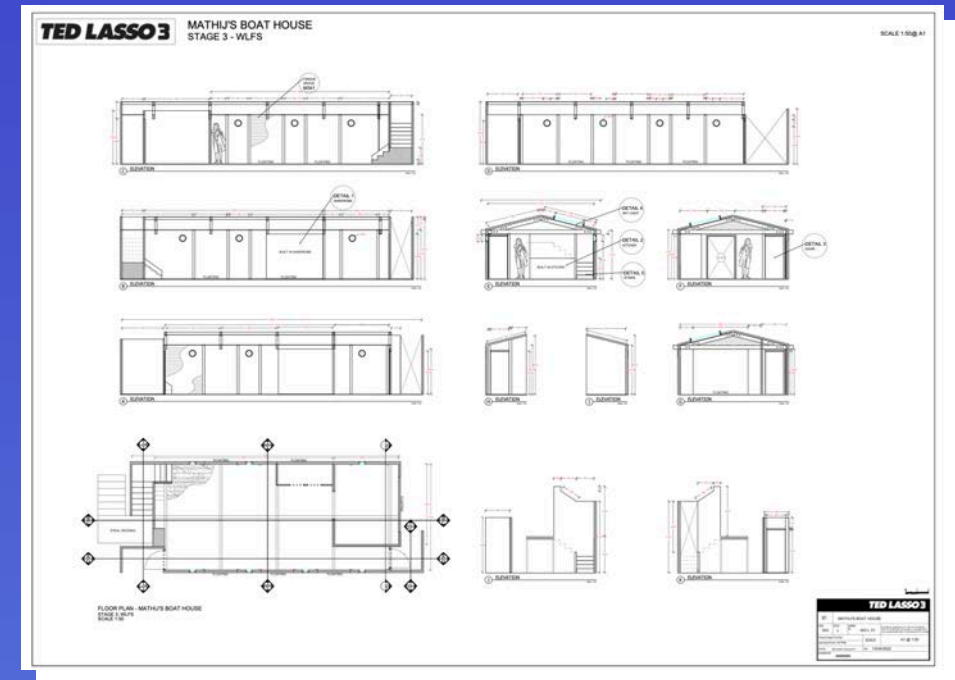
CAD drawings of houseboat studio set
