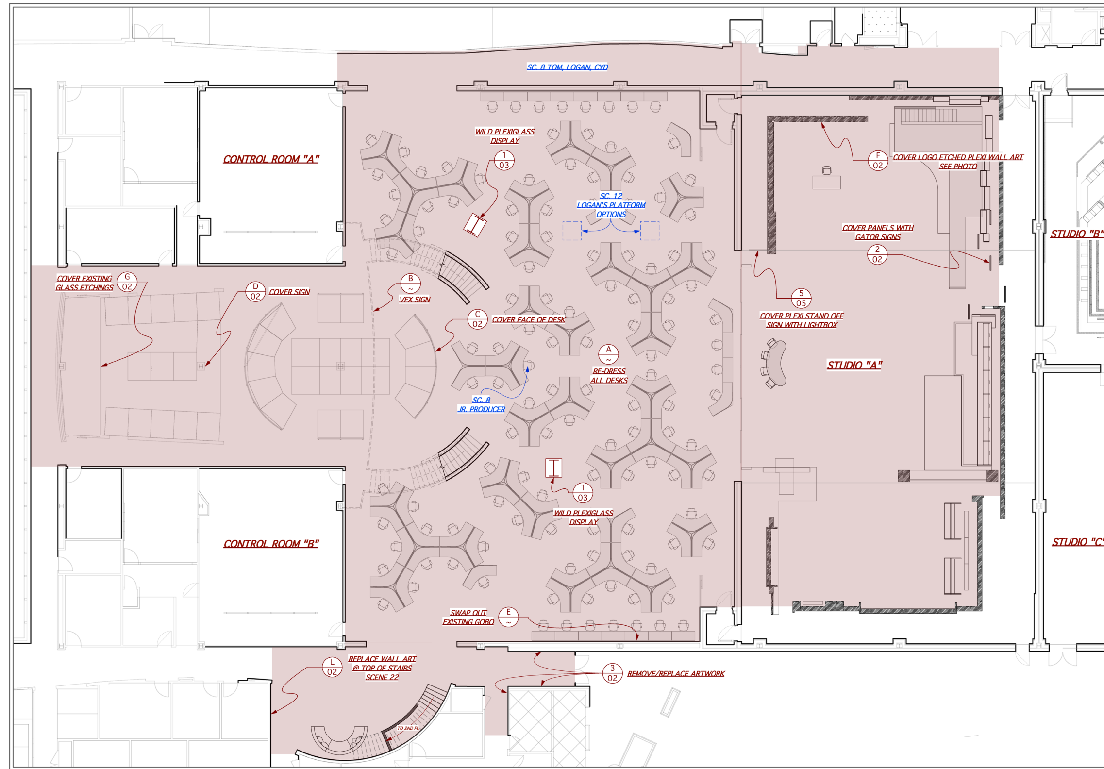
A-A LOCATION PLAN (1ST FLOOR) - INT ATN, BULLPEN, STUDIO Scale: 3/32" = 1'-0"
