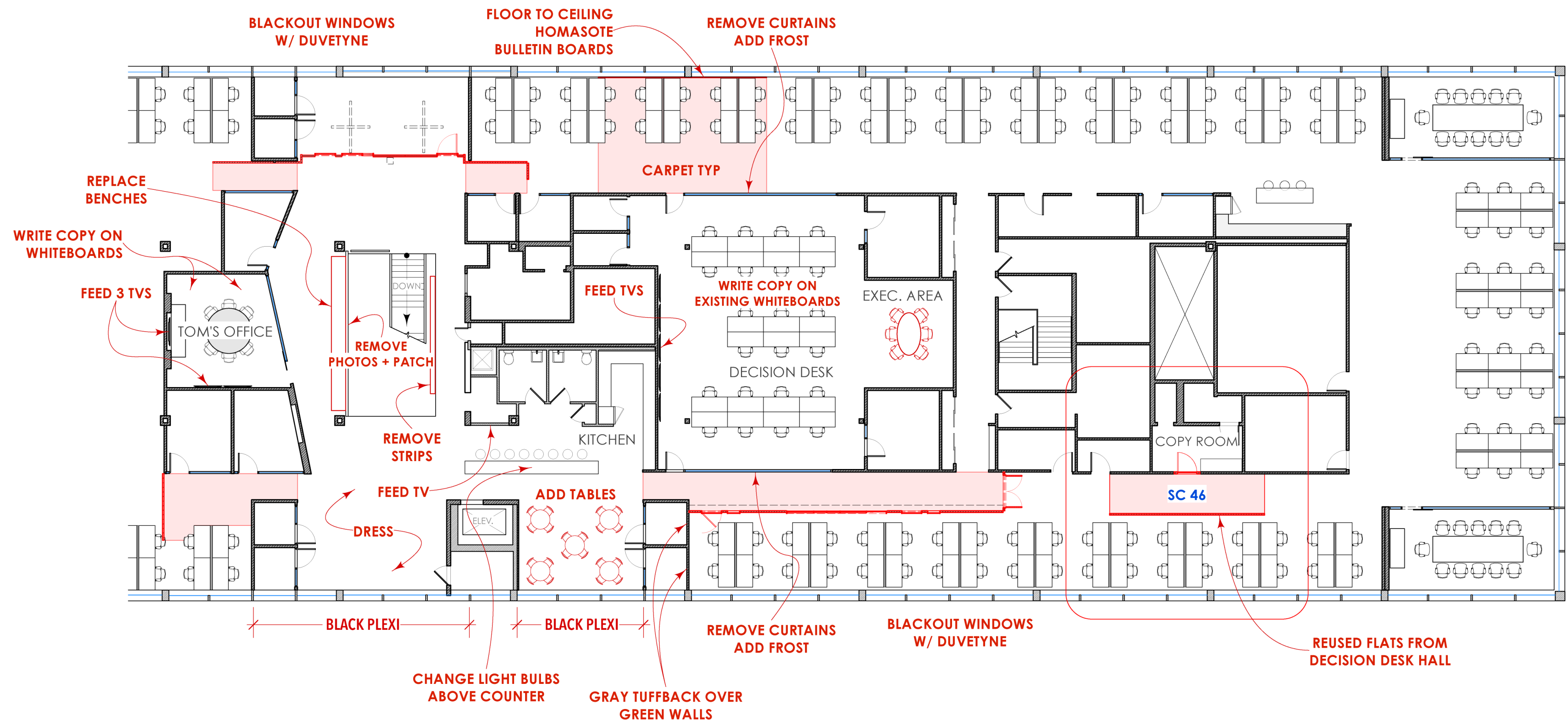
DP INT ATN (NBCU - 2nd FL) Scale: 1/16" = 1'-0"
