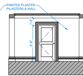
H HALLWAY SECTION SCALE 1/4"=1'-0"
