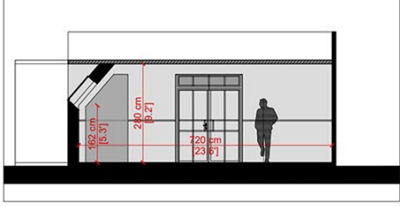
Transversal section 4 / Sc. 1:50
