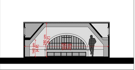
Transversal section 2 / Sc. 1:50
