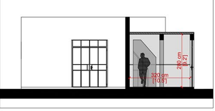
Transversal section 5 / Sc. 1:50
