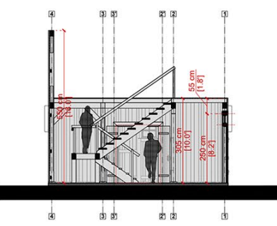
Transversal section 2 / Sc. 1:50
