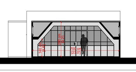
Transversal section 3 / Sc. 1:50
