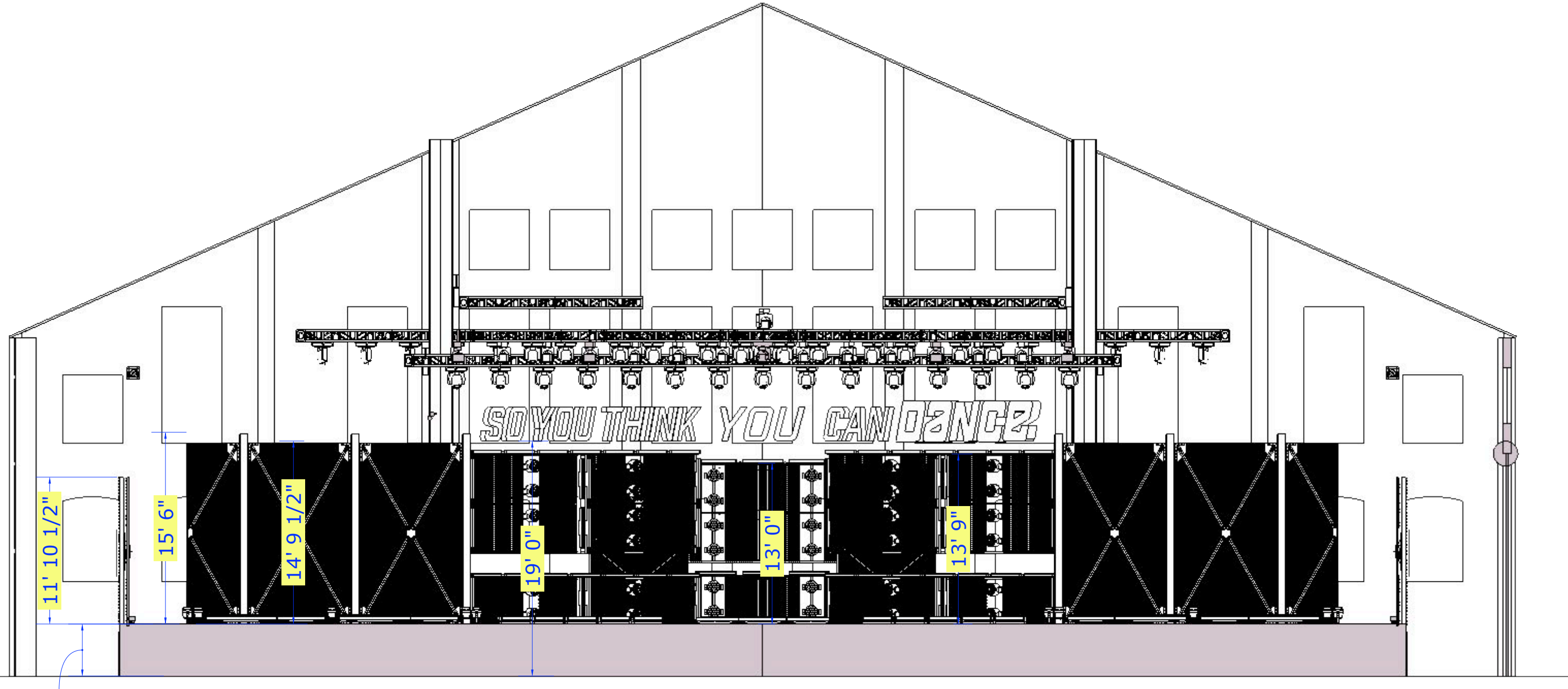
UPSTAGE ELEVATION
