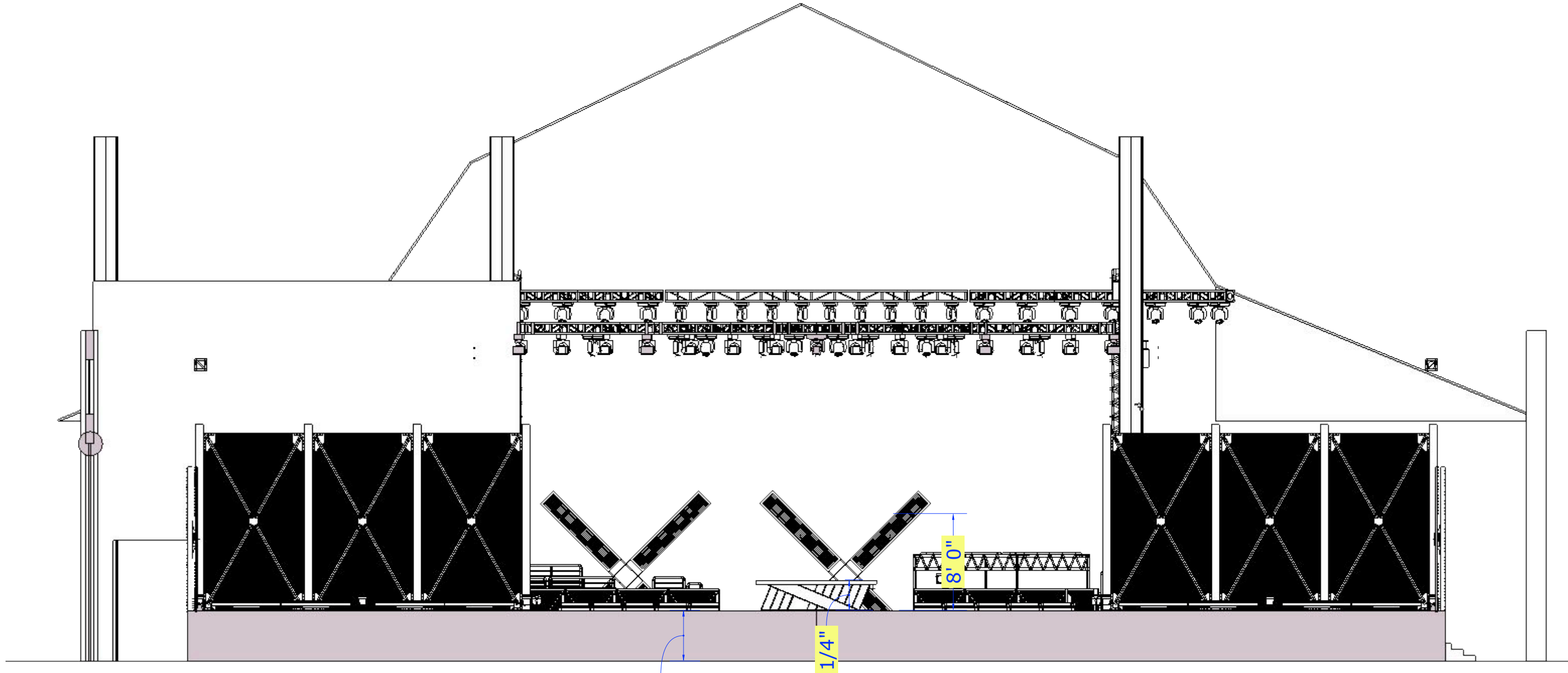
DOWNSTAGE ELEVATION
