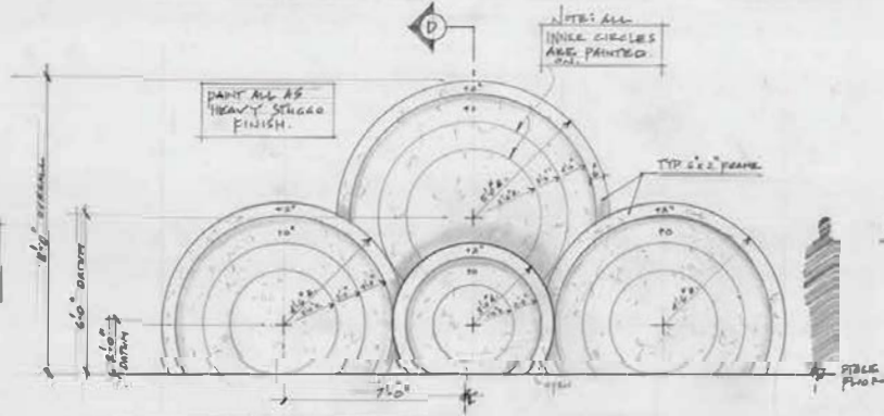
C ELEVATION - BACKING CIRCLES
