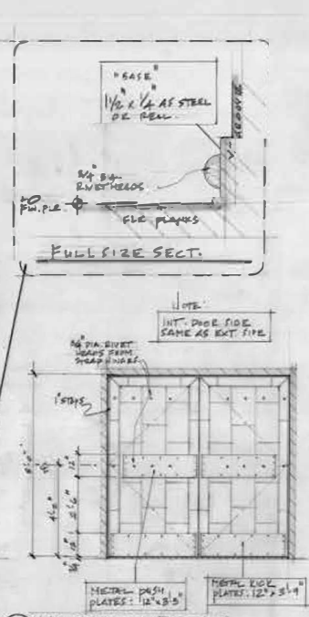
(E) INT. SIDE OF DOORS 1/2" = 10'-0"
