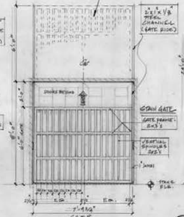
(B) INT. ELEVATION 1/2" = 10'-0"
