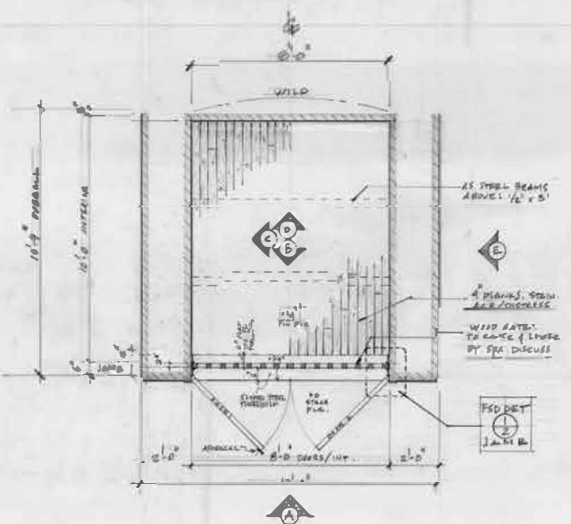
PLAN - INT./EXT. FREIGHT ELEVATOR 1/2" = 10'-0"
