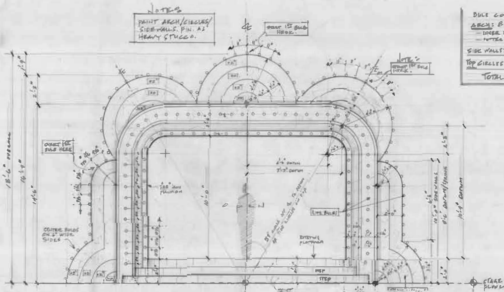
A FRONT ELEVATION
