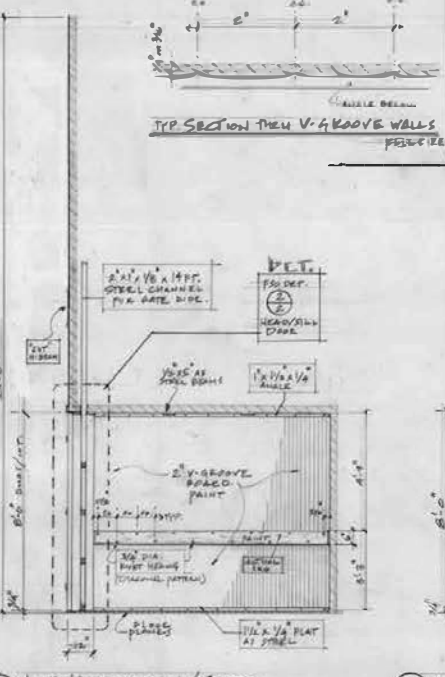
(C) INT. ELEVATION / SECT. 1/2" = 10'-0"
