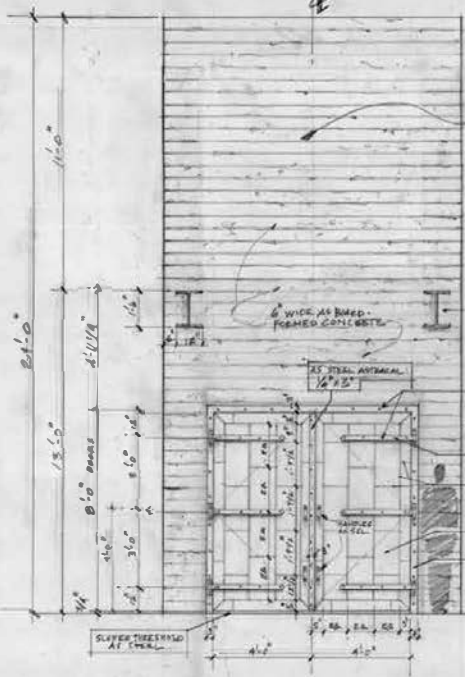
(A) FRONT ELEVATION - SHAFT 1/2" = 10'-0"
