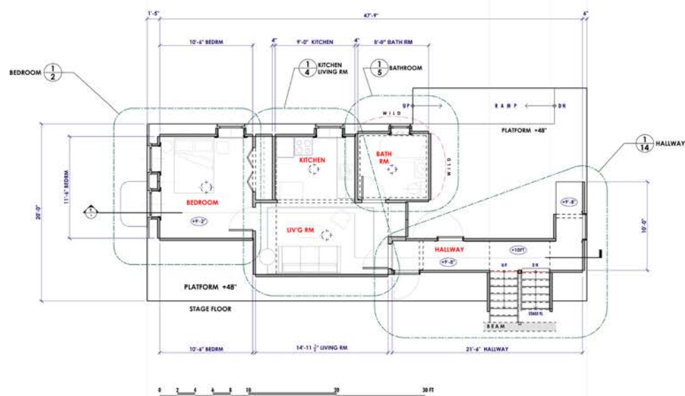
2. PLAN 1/4" = 1' FT
