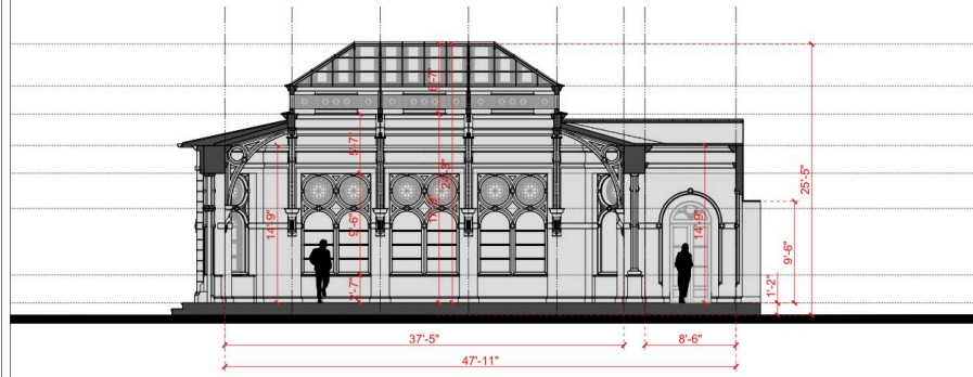
Section S3 - Interior long elevation (side windows) / Scale 1/4":1'
