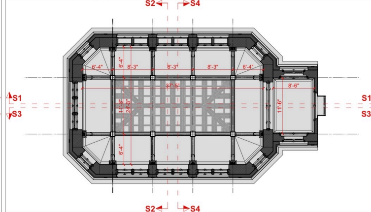
REFLECTED PLAN (Ceiling plan) / Scale 1/4":1'
