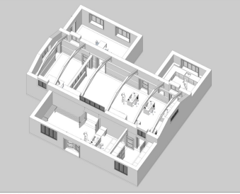
ISOMETRIC MODEL VIEWS
