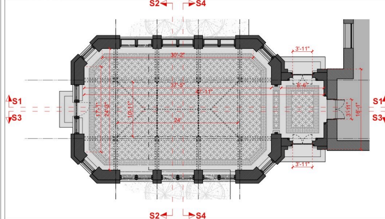
PLAN / Scale 1/4":1'
