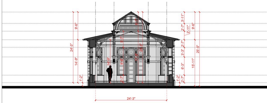
Section S4 - Interior short elevation (french doors entrance) / Scale 1/4":1'
