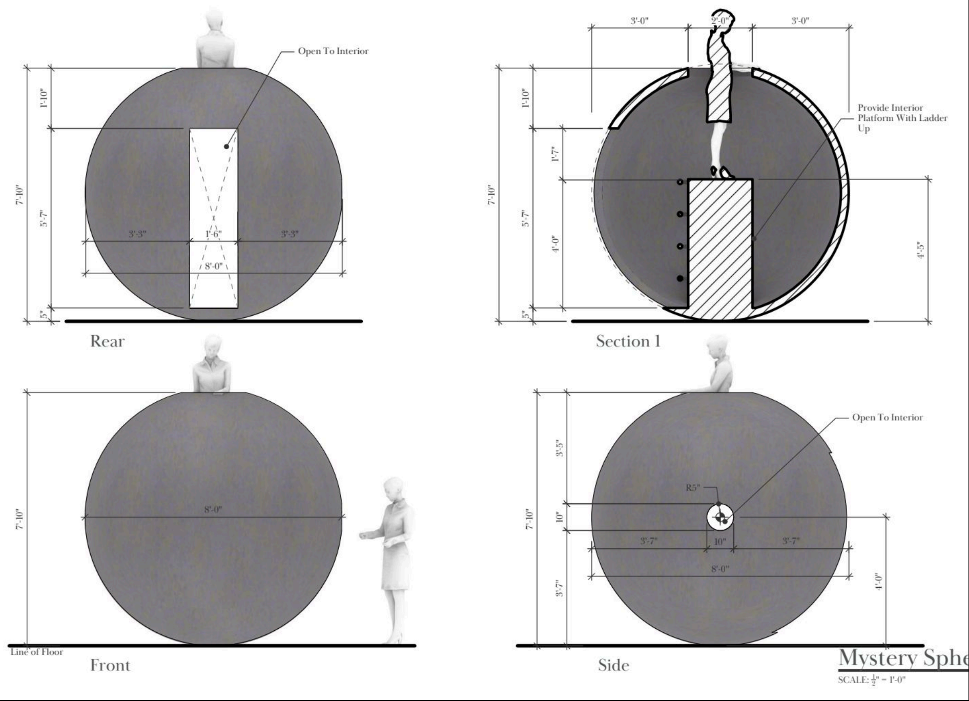
SET DRAWINGS
