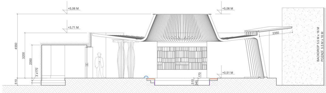
SECTION B - B REZ B - B 1:50_A0
