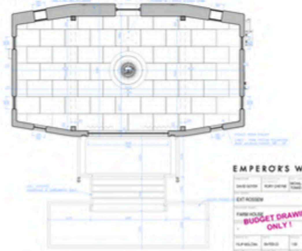
FLOOR PLAN
