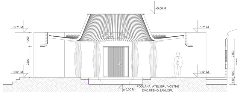
SECTION D - D REZ D - D 1:50_A0
