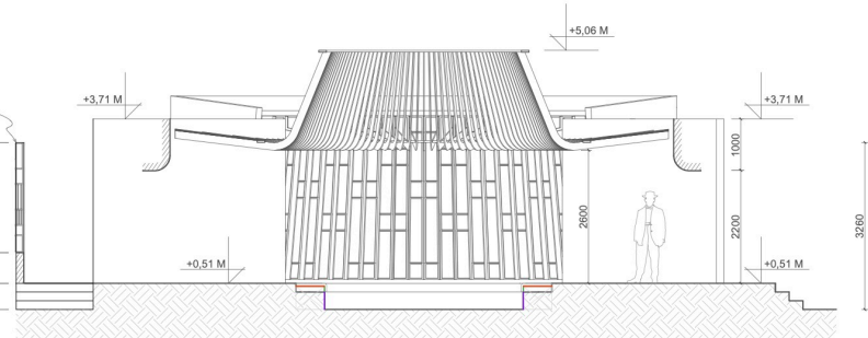
SECTION C - C REZ C - C 1:50_A0
