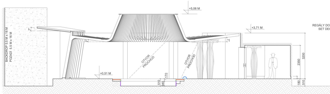
SECTION A - A REZ A - A 1:50_A0
