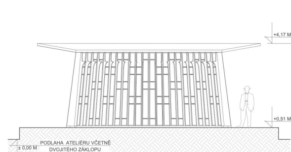
SECTION F - F REZ F - F 1:50_A0
