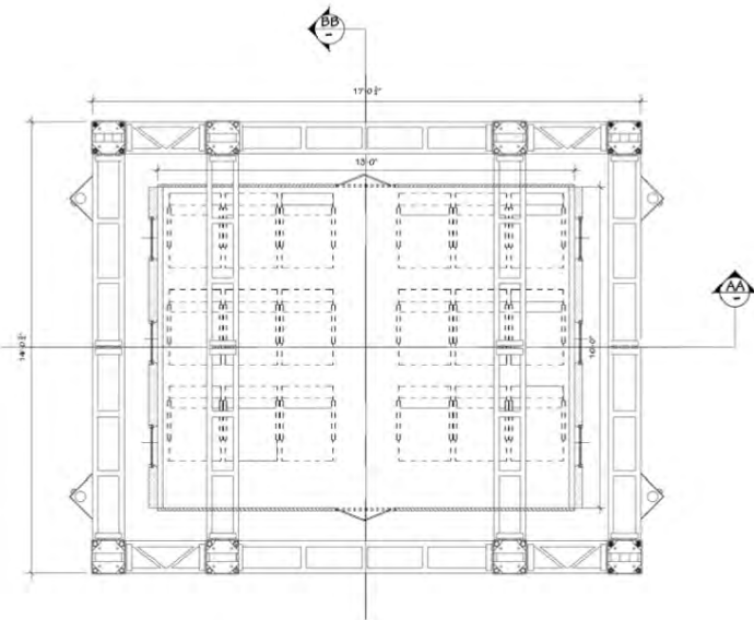
PLAN VIEW 1/2"=1'-0"
