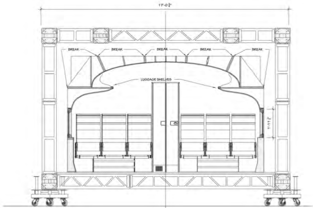
AA SECTION VIEW THRU AA 1/2"=1'-0"
