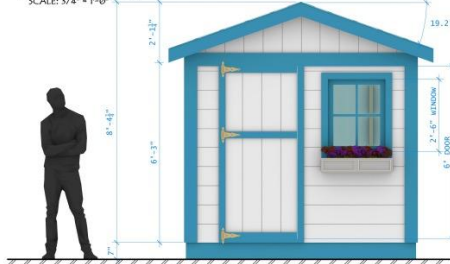
FRONT ELEVATION SCALE: 3/4" = 1'-0"
