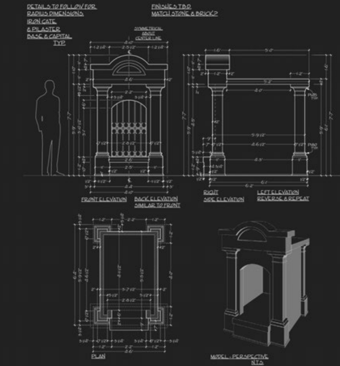
GRAVE YARD-CRYPT PLAN & ELEVATIONS
