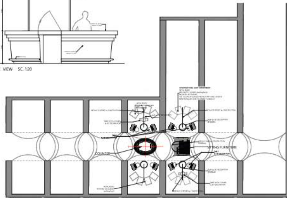
PLAN SC. 1:100
