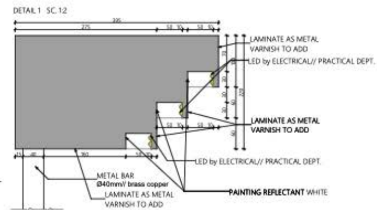
DETAIL 1 SC. 1:2
