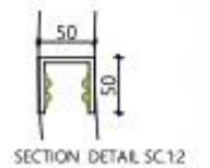
SECTION DETAIL SC. 1:2
